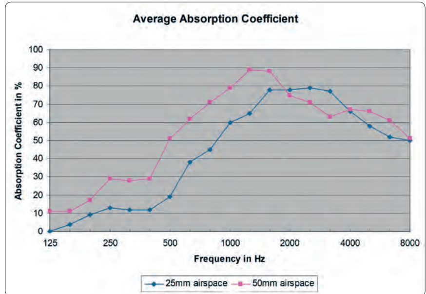
Average absorption coefficient of the MayTec 1-layer "Noise Resist"
